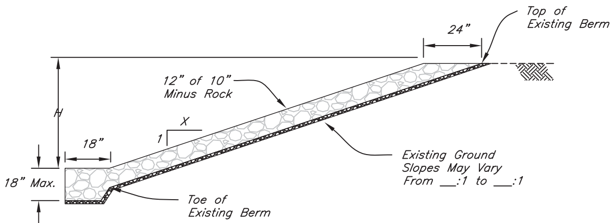
SECTION VIEW
